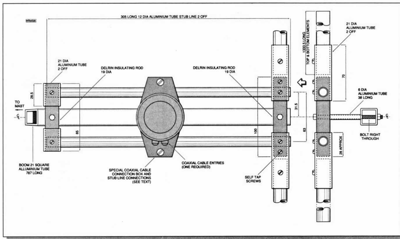
Fig.3: Constructional details, dimensions and materials for the assembly of the twin stub line with the driven elements and the position of the cable connection housing (see text regarding availability of this unit).
