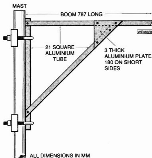
Fig.6: Suggested arrangement for supporting the boom and antenna and attachment to a metal or wood mast.
