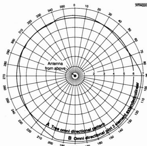
Fig.7: Plot A. Perfect circular omni-directional radiation pattern. Plot B. From the vertical extended collinear. Slight deviation due to other nearby vertical 2m antennas, proximity of metal mast and other conductors. The 3/8ths wavelength offset provided by the boom is about optimum and should not be less.
