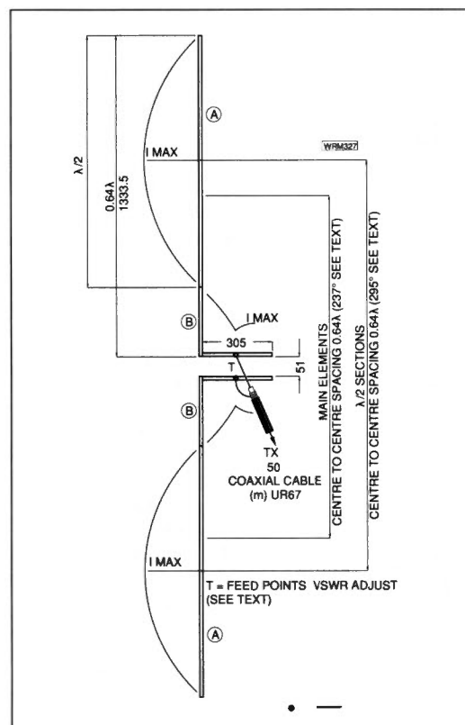
Fig.1: Configuration, general dimensions, current distribution, etc. 2-element extended collinear antenna.
